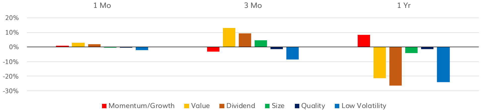
Factor Relative Performance to SPY
