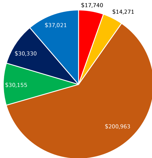
U.S. Factor AUM
