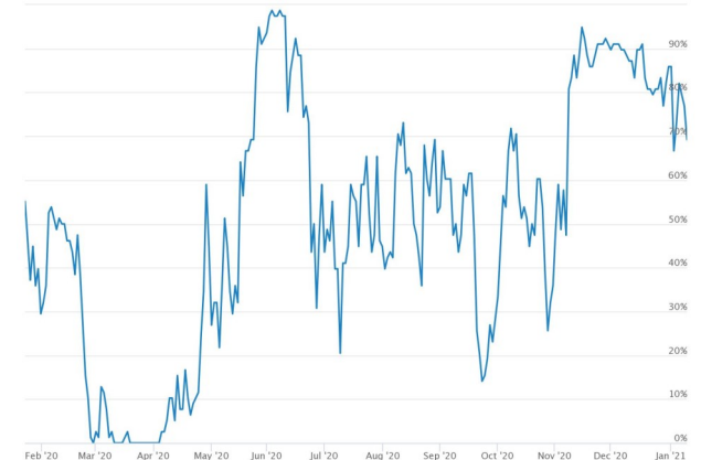
Holdings Above 50 DMA (RSP)
