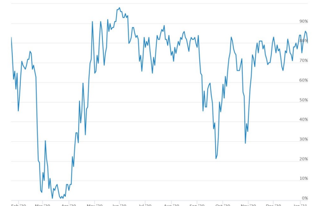
Holdings Above 50 DMA (SPHQ)
