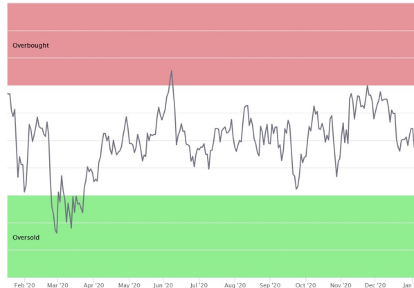
14 Day RSI (RSP)
