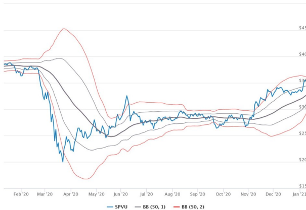
50 Day Bollinger Bands (SPVU)
