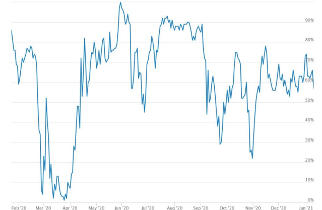
Holdings Above 50 DMA (SPLV)
