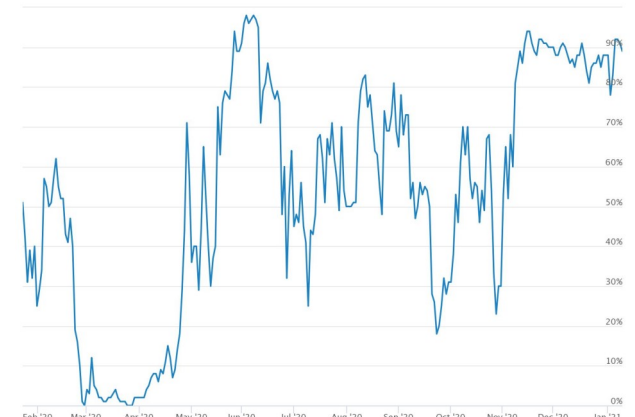
Holdings Above 50 DMA (SPVU)
