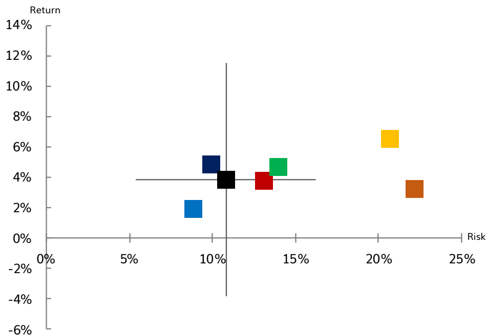
One Month Dispersion
