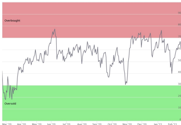
Holdings Above 50 DMA (VEA)
